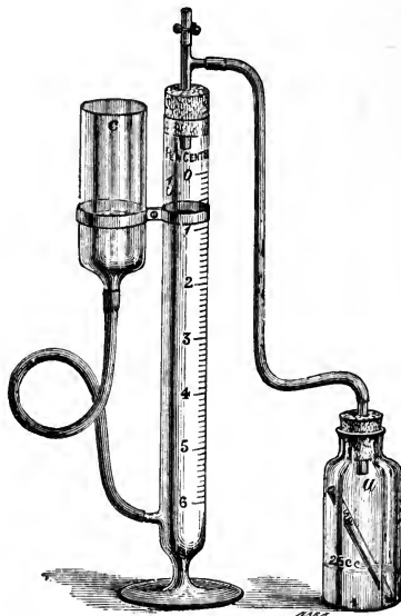
Fig. 10.—GERRARD'S UREOMETER.
